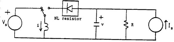
Figure 1: Up-Down Converter Redrawn to Illustrate Stability in Case of Discontinuous Conduction
