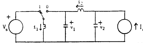
Figure 5: Up-Down Converter with Additional Filter Sections
