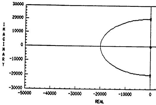
Figure 3: Root-Locus for Linearized Closed-Loop Control System
